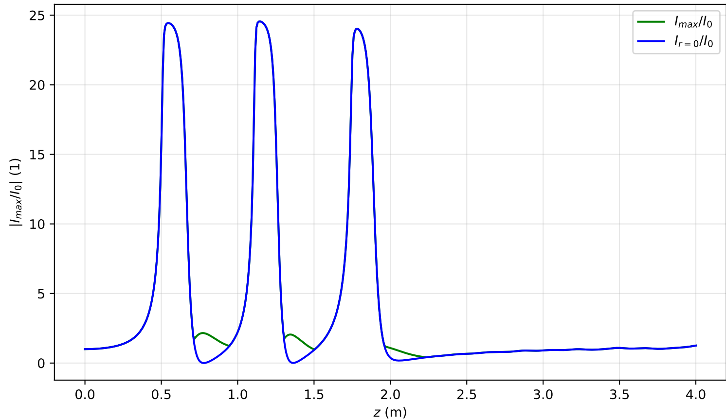
I_{max}(x = 0, y = 0, z)/I_0 , \text{Pin}=4.5\text{Pcr} , artificial time
